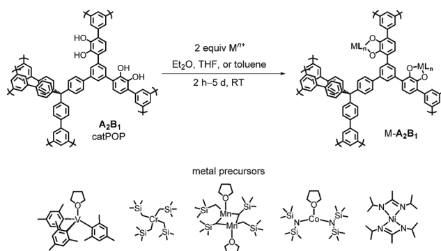
Scheme 1. General metallation procedure of catPOP A_2B_1 . The notation A_2B_1 refers to the ratio of the two comonomers used to synthesize the POP ( A = catechol structure, B = tetraphenylmethane node).
